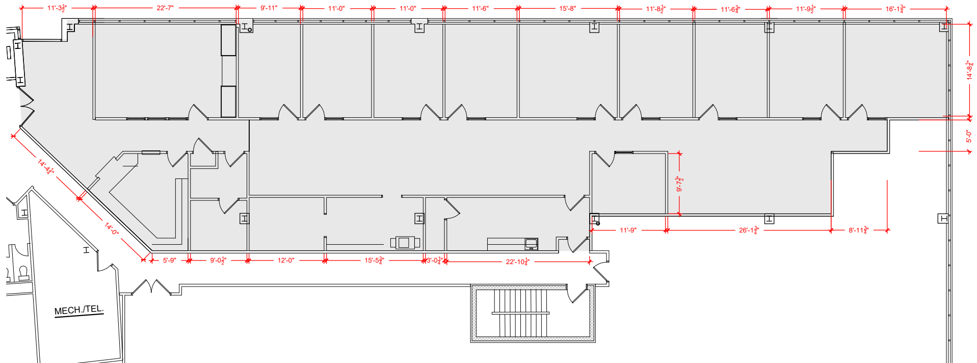
Floor Plan
